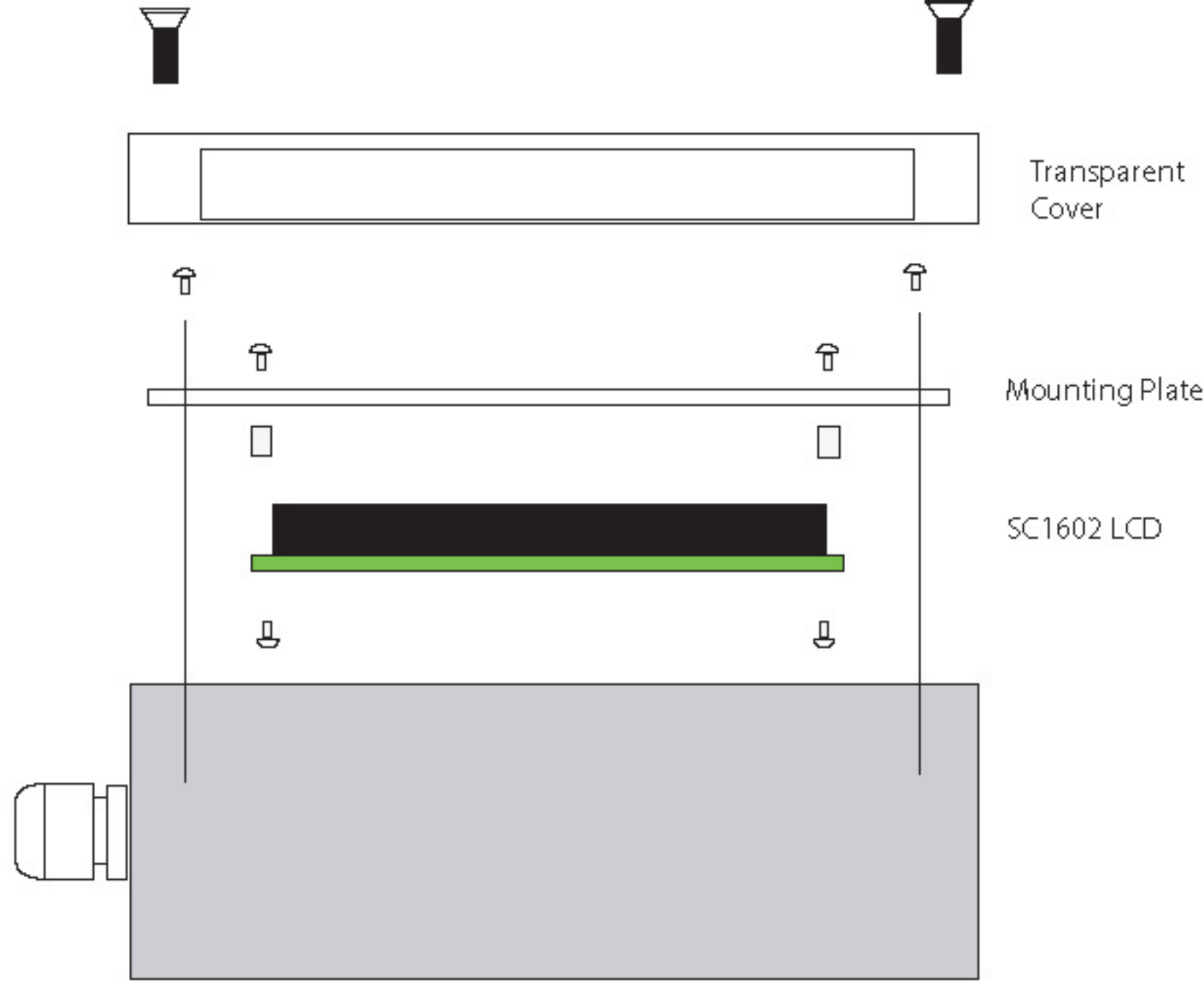
Mounting SC1602 LCD to SC1602ENIP65 Enclosure
